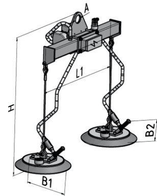
Vario handling façade elements
